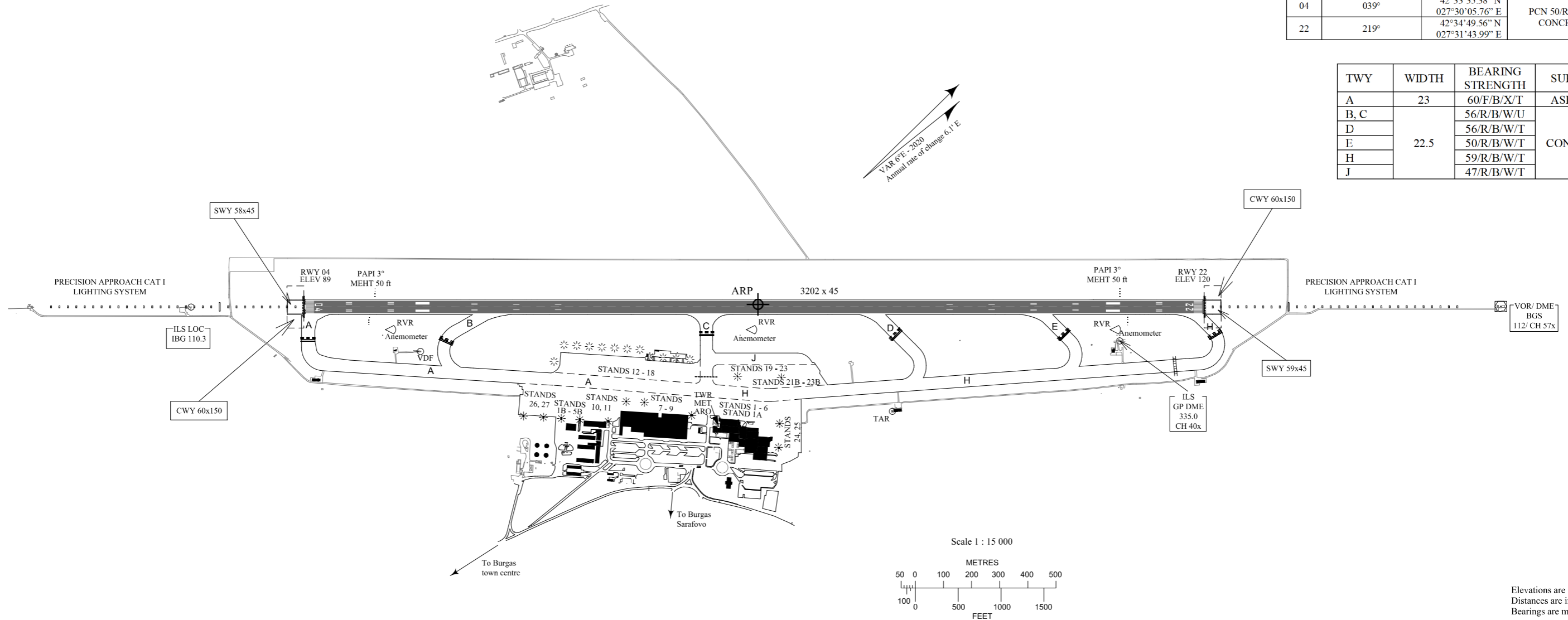
LIGHTING AIDS RWY 04/22 AND EXIT TWY
