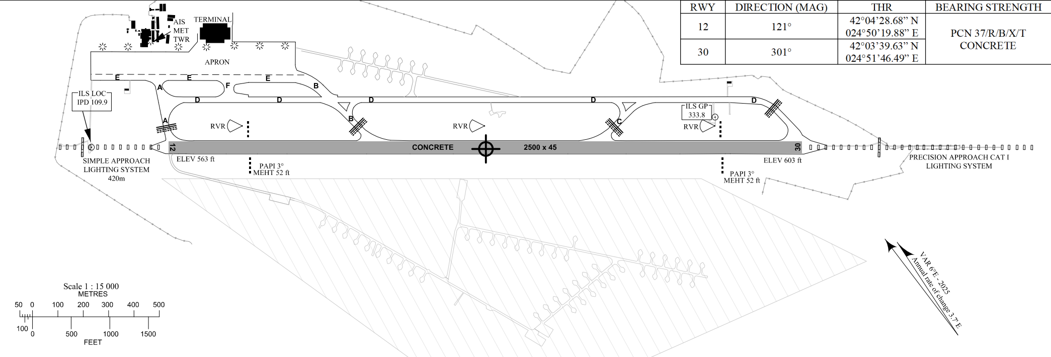
LIGHTING AIDS RWY 12/30 AND EXIT TWY
