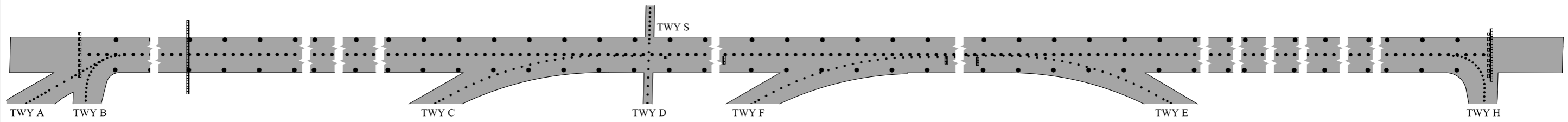
LIGHTING AIDS RWY 09/27 AND EXIT TWY (TDZ lighting not shown)
